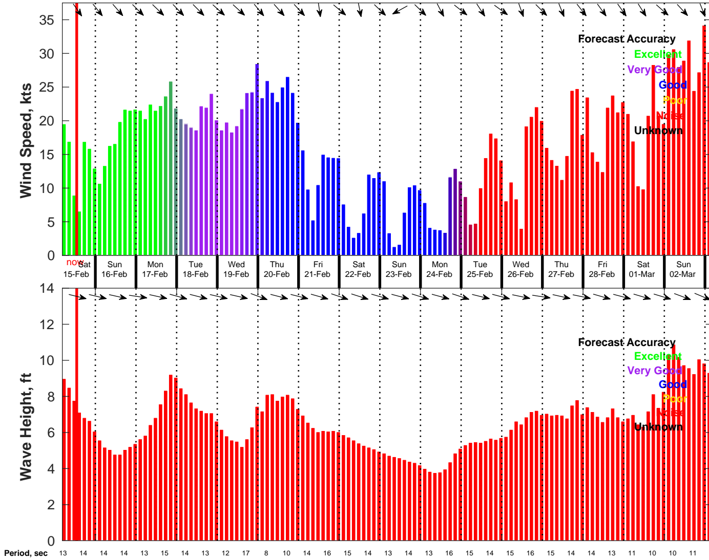
Wind & Wave Forecast for NDBC 46054 from 15-Feb-2025 04:00:00 to 03-Mar-2025 04:00:00
