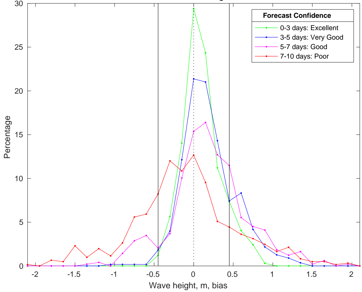
NDBC 46069 vs CMEMS Waves Bias Histogram: 15-Feb-2025
