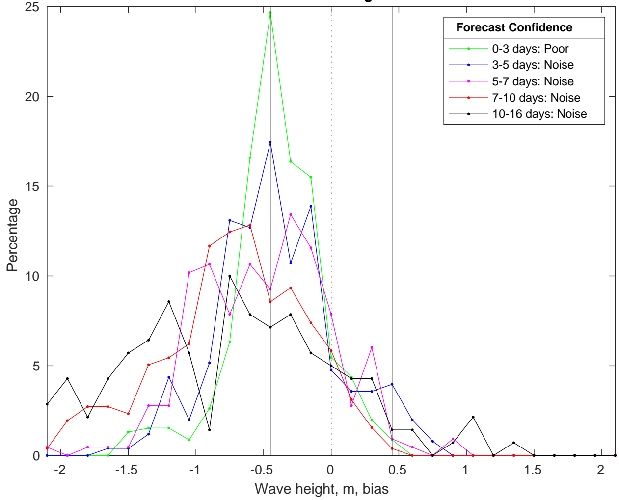
NDBC 46069 vs GFS Waves Bias Histogram: 15-Feb-2025
