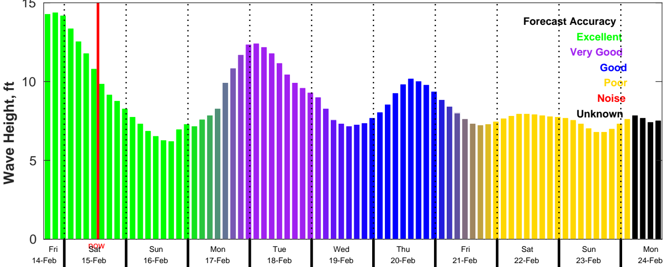
CMEMS Wave Forecast for NDBC 46069 from 14-Feb-2025 16:00:00 to 24-Feb-2025 16:00:00
