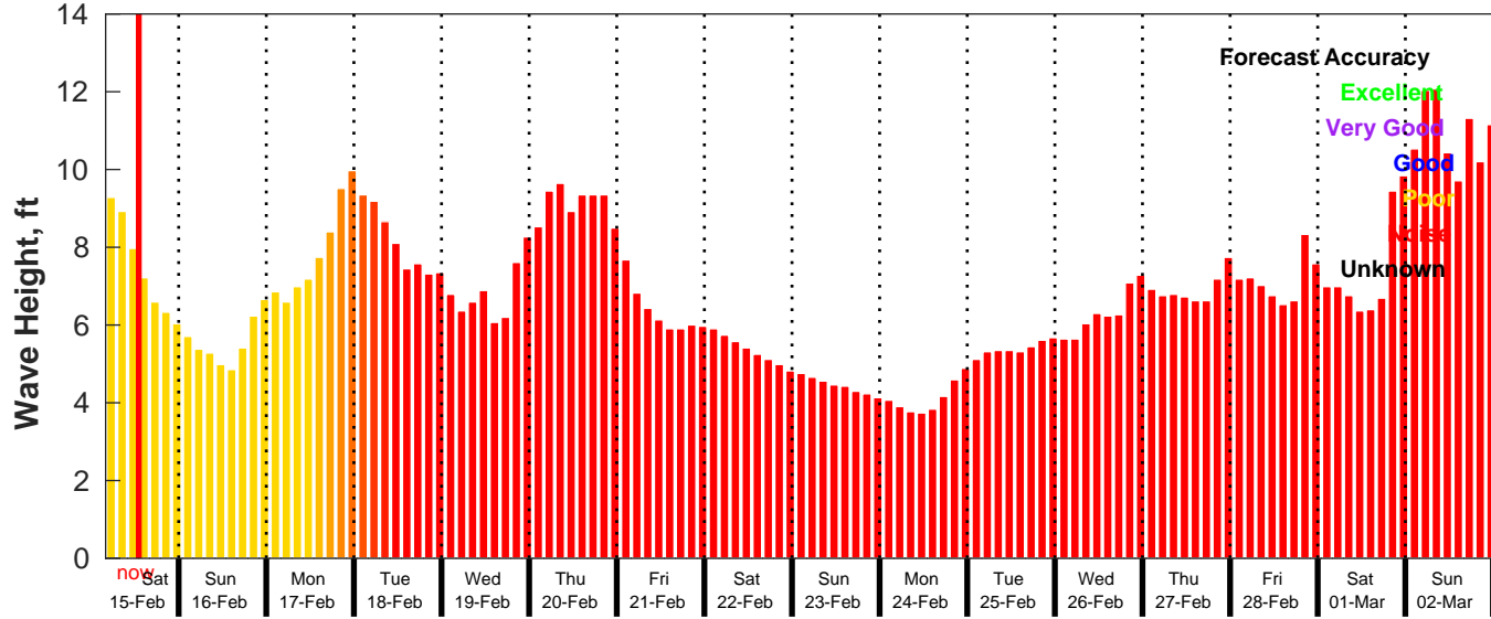
GFS Wave Forecast for NDBC 46069 from 15-Feb-2025 04:00:00 to 03-Mar-2025 04:00:00
