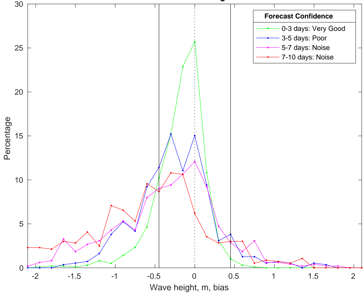
NDBC 46246 vs CMEMS Waves Bias Histogram: 15-Feb-2025
