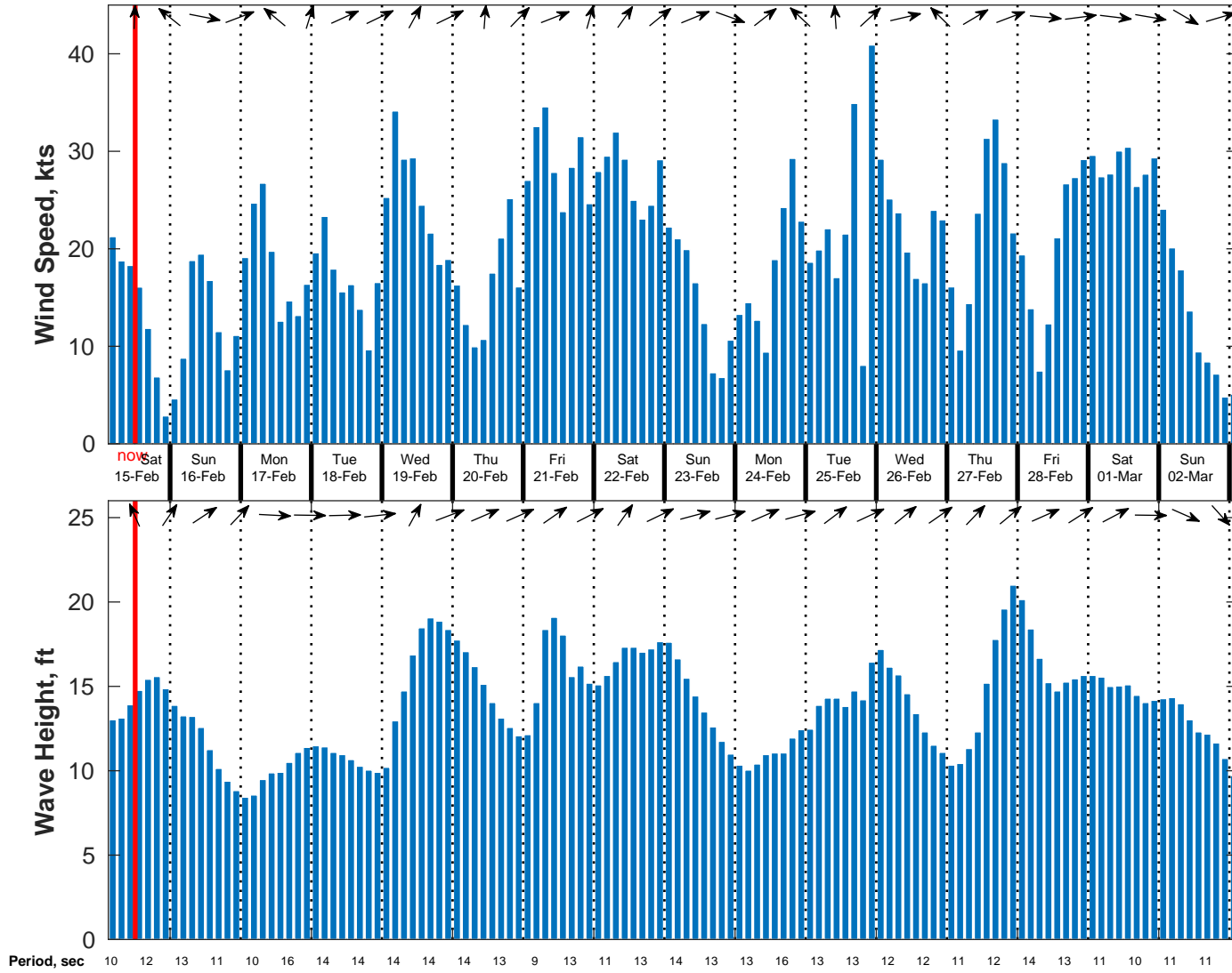
Wind & Wave Forecast for NDBC 46246 from 15-Feb-2025 03:00:00 to 03-Mar-2025 03:00:00
