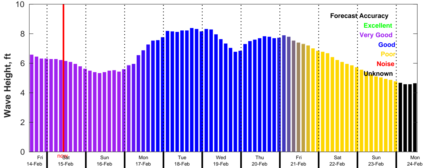
CMEMS Wave Forecast for NDBC 51209 from 14-Feb-2025 13:00:00 to 24-Feb-2025 13:00:00
