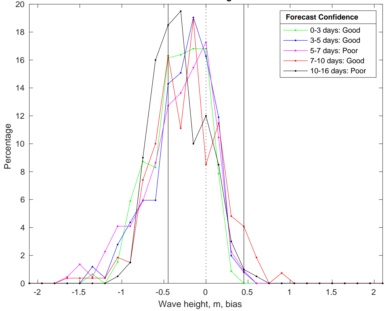
NDBC 52211 vs GFS Waves Bias Histogram: 15-Feb-2025
