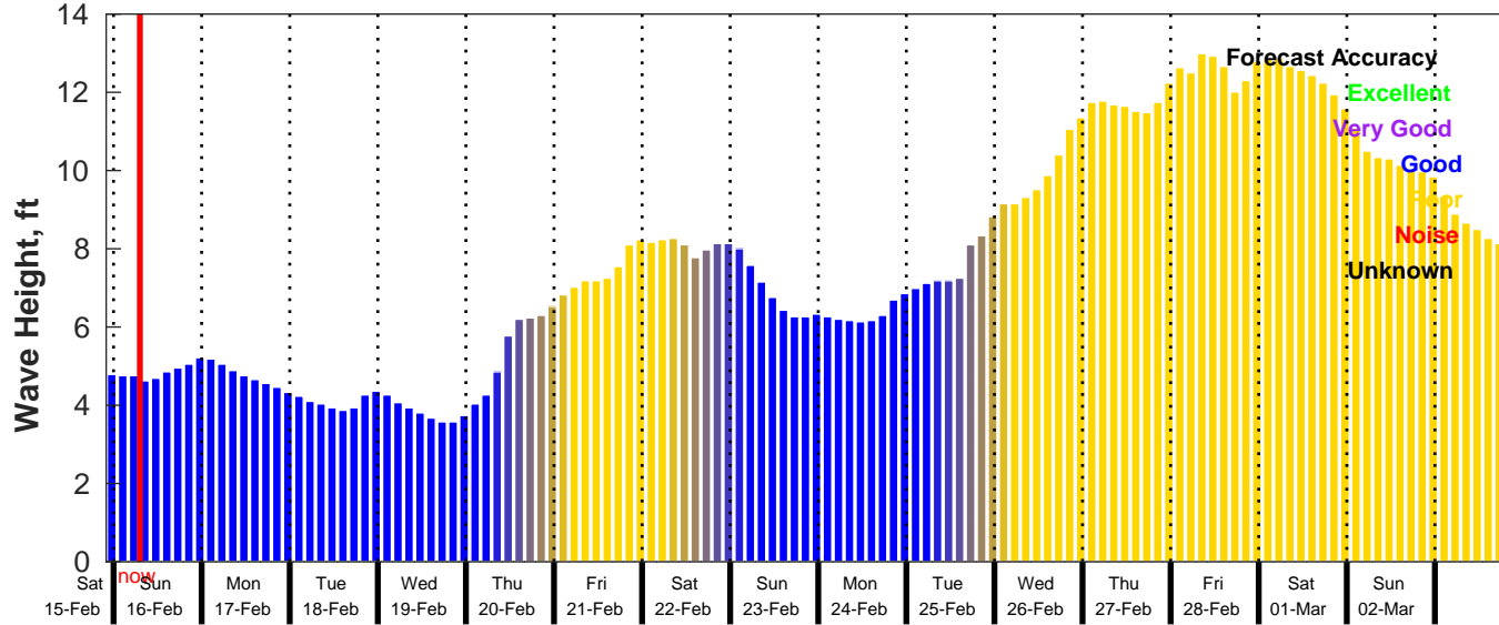
GFS Wave Forecast for NDBC 52211 from 15-Feb-2025 22:00:00 to 03-Mar-2025 22:00:00
