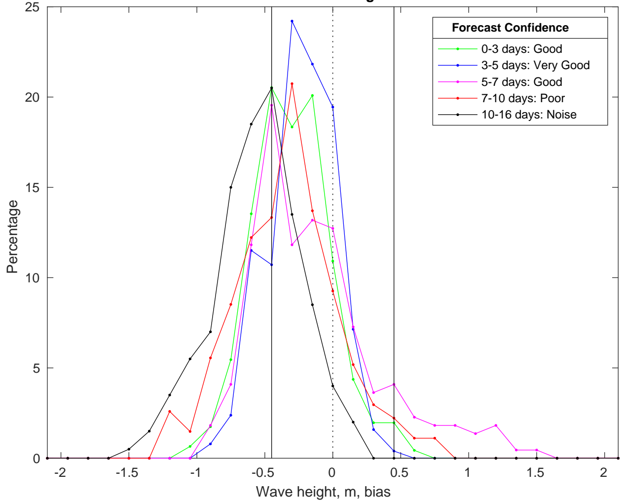
NDBC 52212 vs GFS Waves Bias Histogram: 15-Feb-2025
