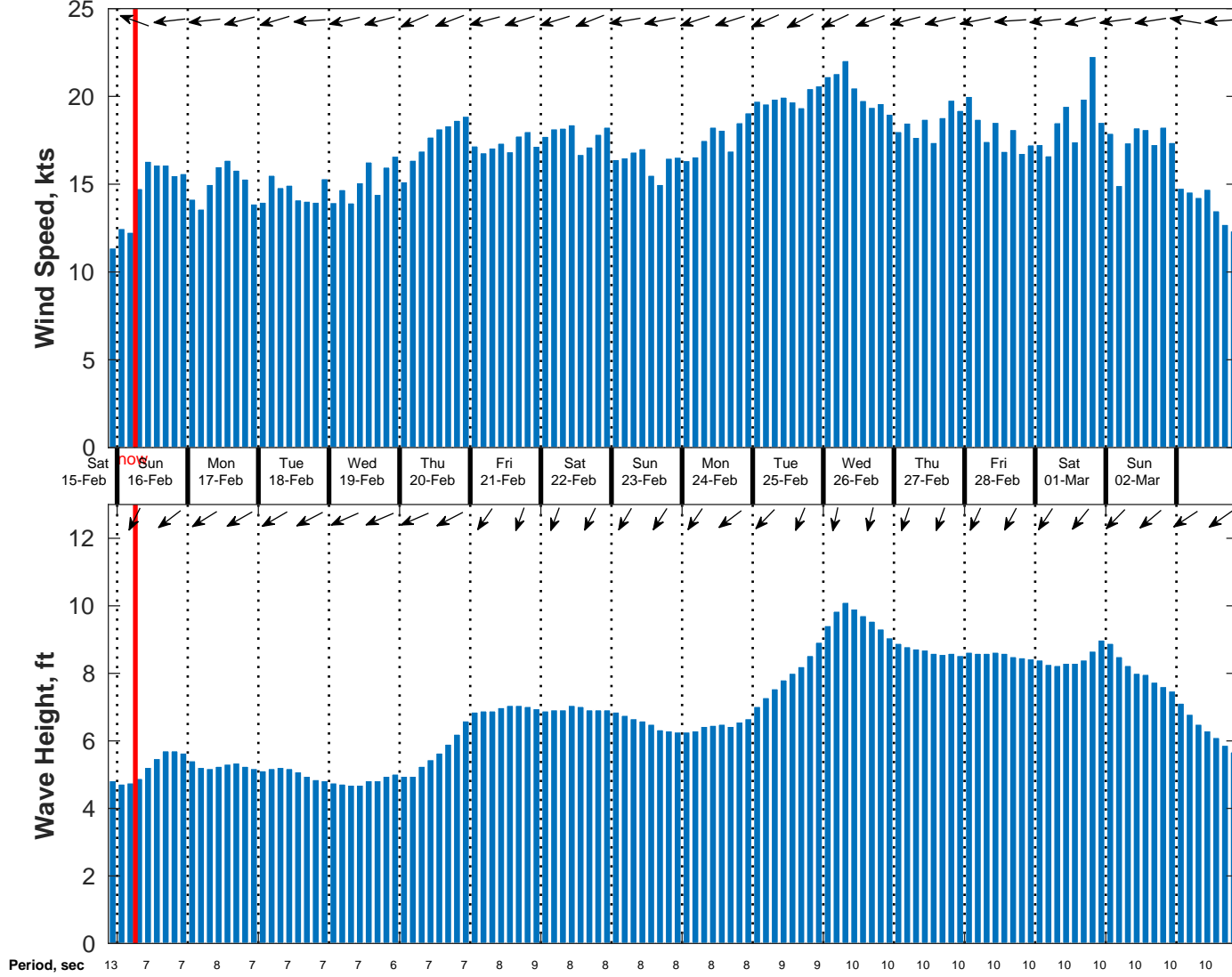
Wind & Wave Forecast for NDBC 52212 from 15-Feb-2025 21:00:00 to 03-Mar-2025 21:00:00
