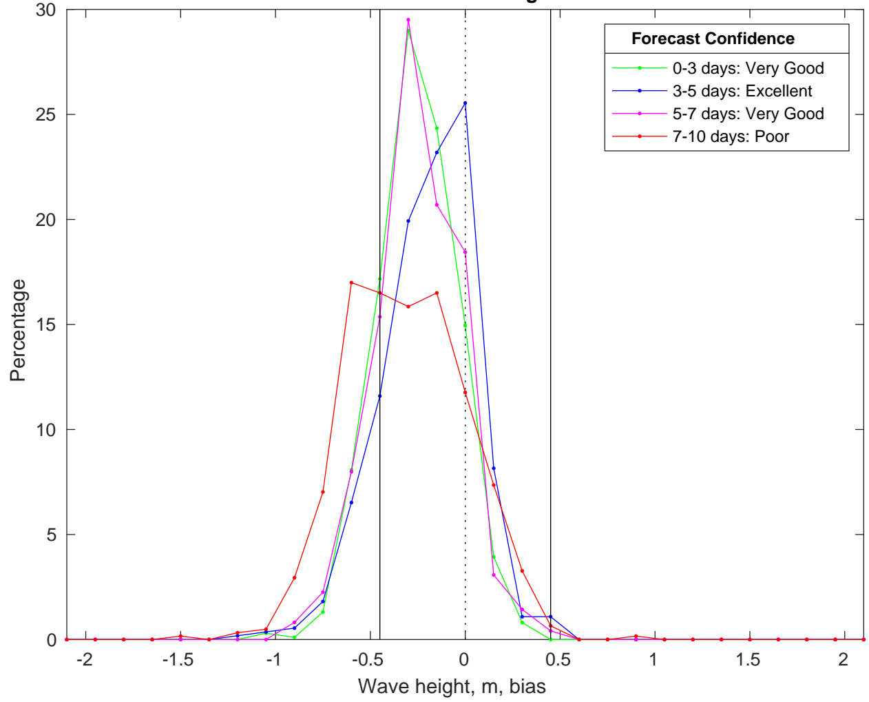
NDBC 52213 vs CMEMS Waves Bias Histogram: 15-Feb-2025
