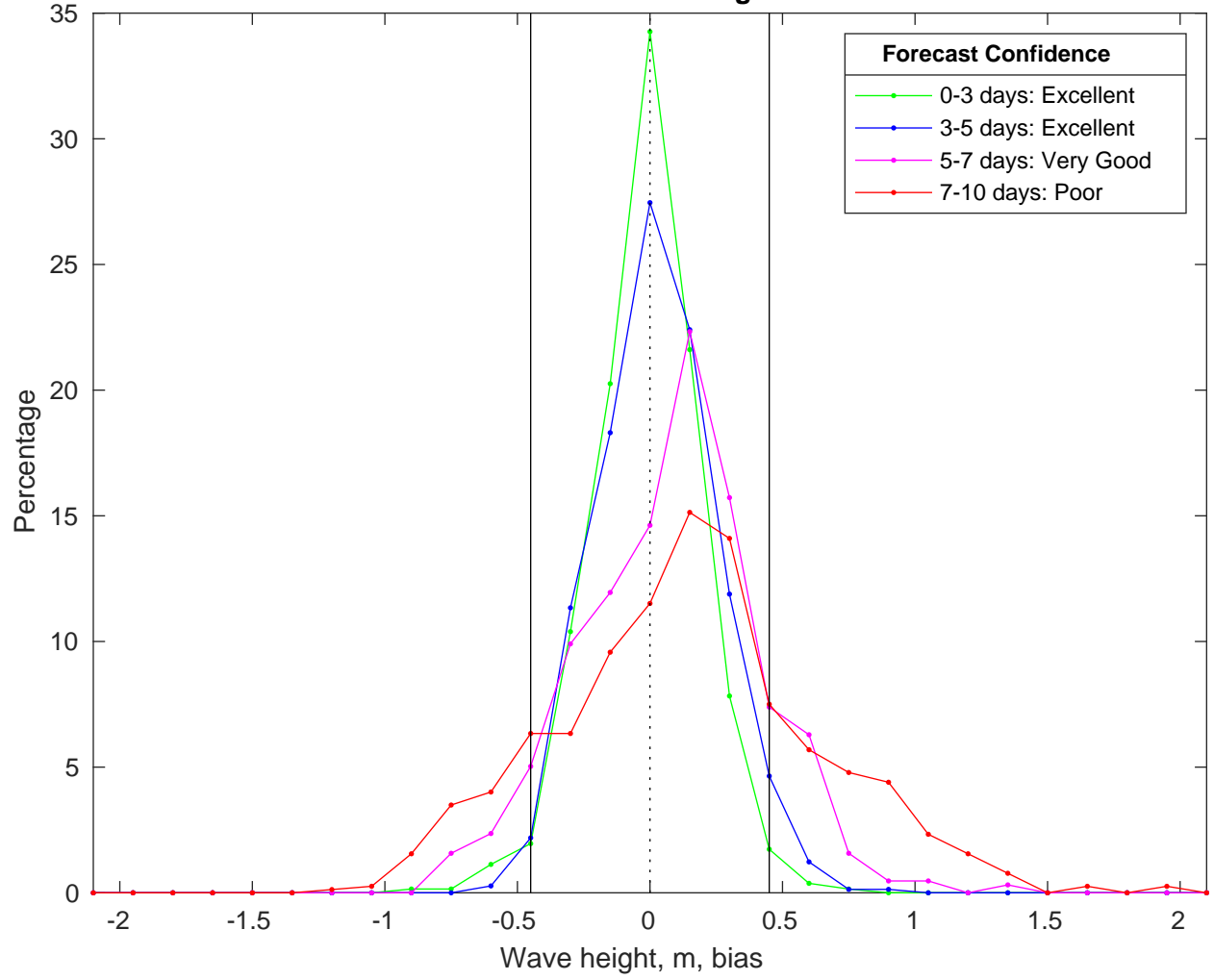
NDBC 41004 vs CMEMS Waves Bias Histogram: 16-Feb-2025
