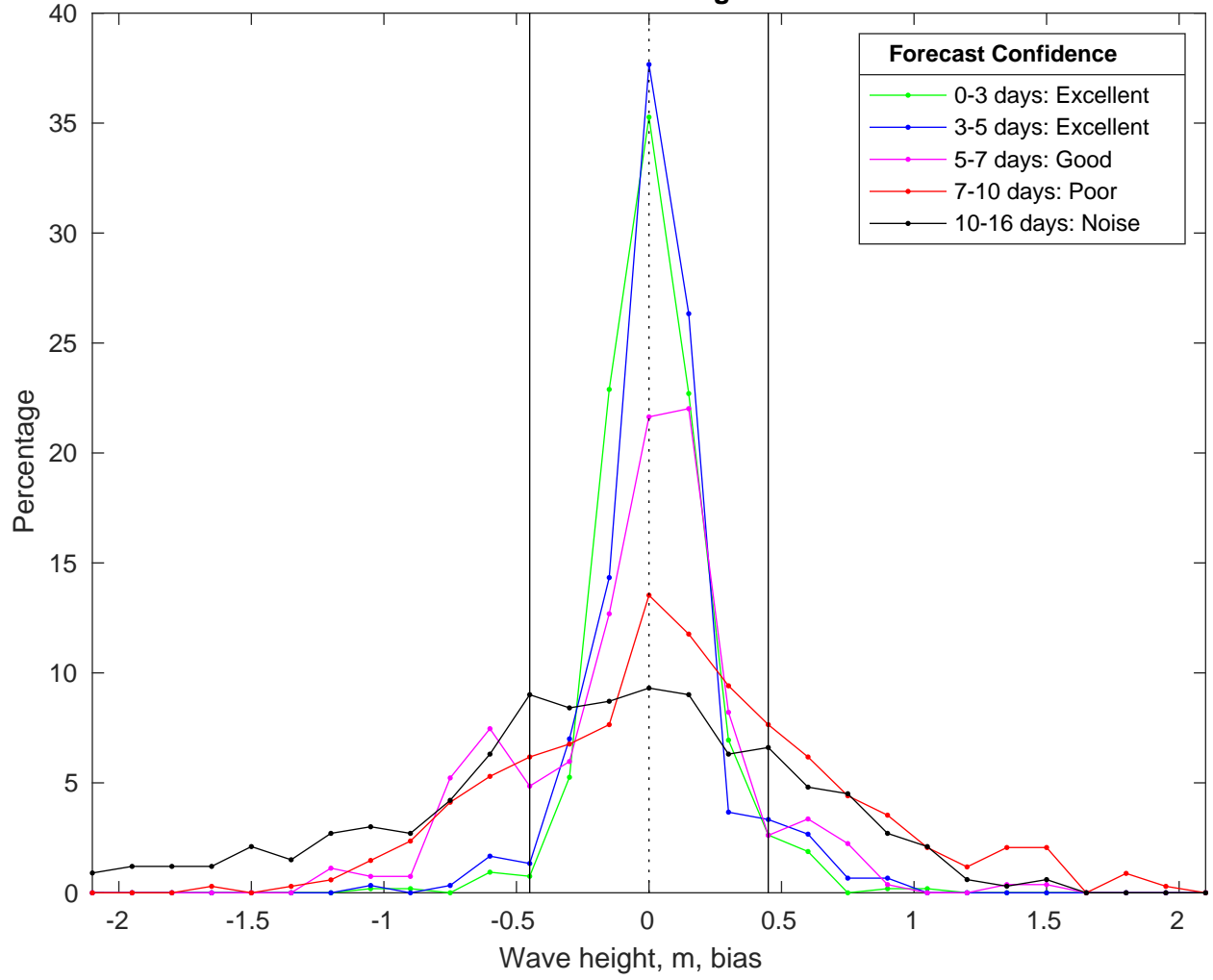
NDBC 41004 vs GFS Waves Bias Histogram: 16-Feb-2025
