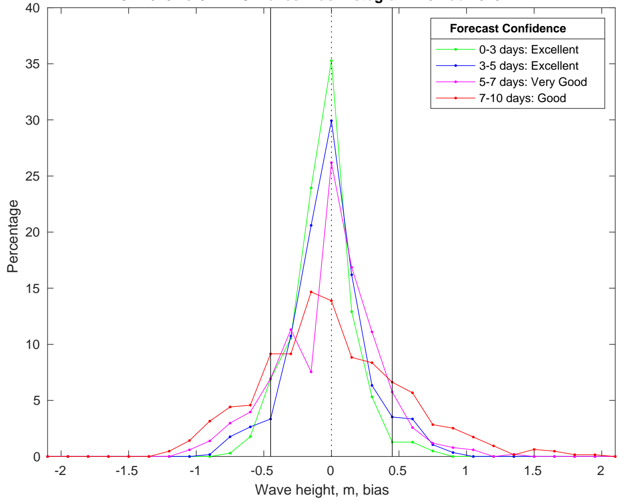
NDBC 41013 vs CMEMS Waves Bias Histogram: 16-Feb-2025
