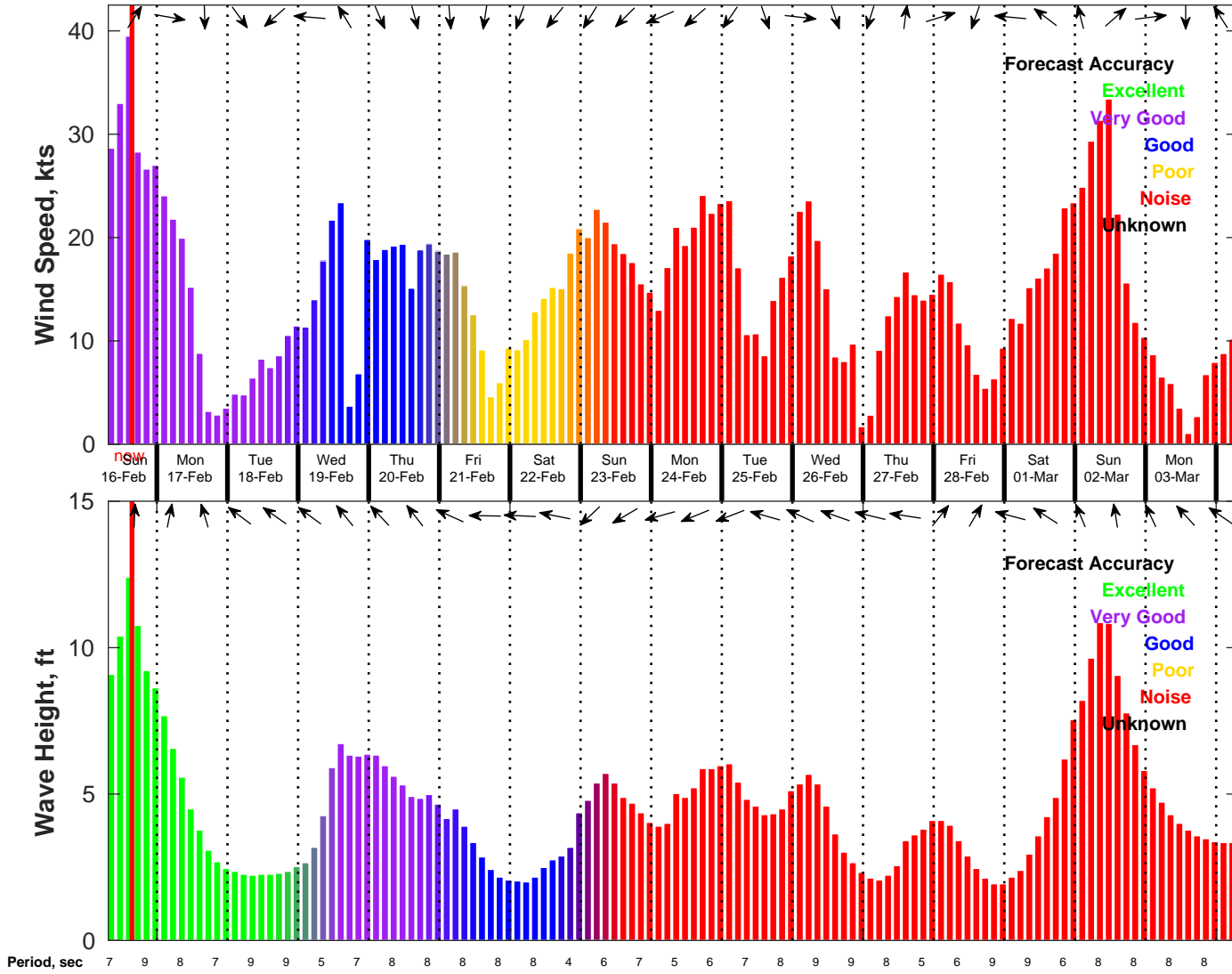
Wind & Wave Forecast for NDBC 41013 from 16-Feb-2025 07:00:00 to 04-Mar-2025 07:00:00
