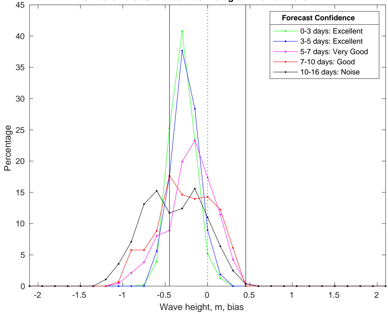
NDBC 41040 vs GFS Waves Bias Histogram: 16-Feb-2025
