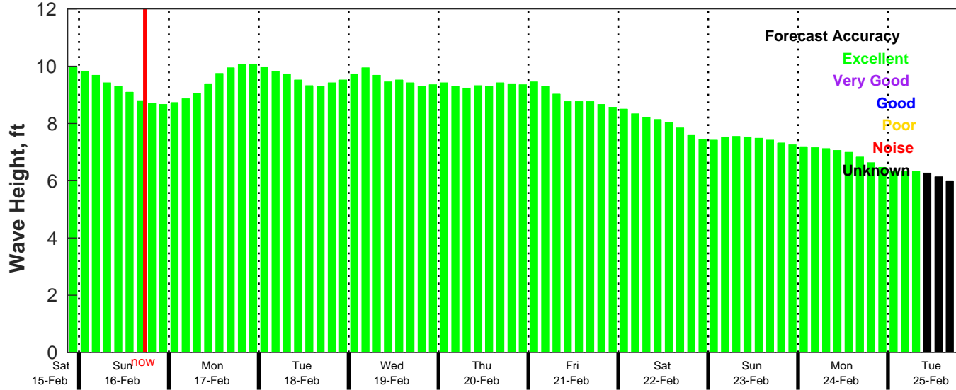
CMEMS Wave Forecast for NDBC 41040 from 15-Feb-2025 21:00:00 to 25-Feb-2025 21:00:00
