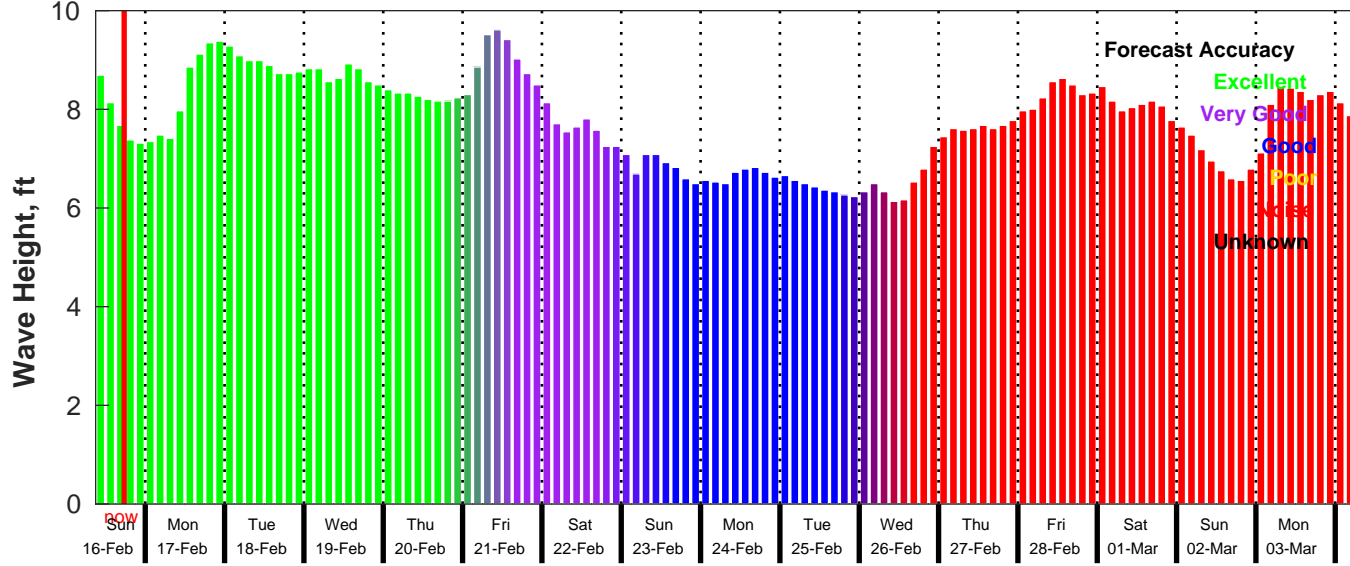
GFS Wave Forecast for NDBC 41040 from 16-Feb-2025 09:00:00 to 04-Mar-2025 09:00:00
