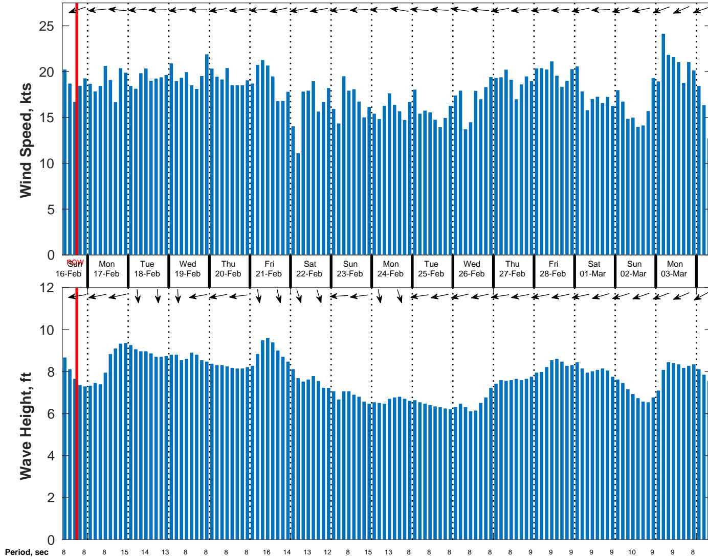
Wind & Wave Forecast for NDBC 41040 from 16-Feb-2025 09:00:00 to 04-Mar-2025 09:00:00
