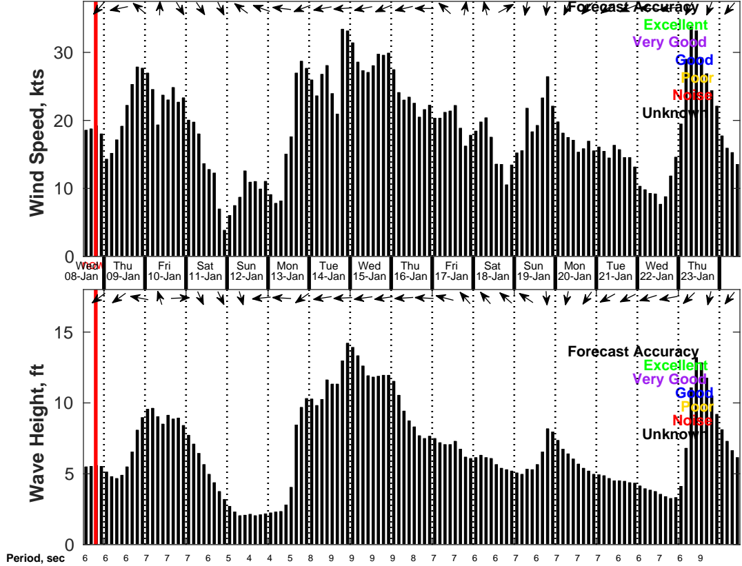
Wind & Wave Forecast for NDBC 42002 from 08-Jan-2025 12:00:00 to 24-Jan-2025 12:00:00
