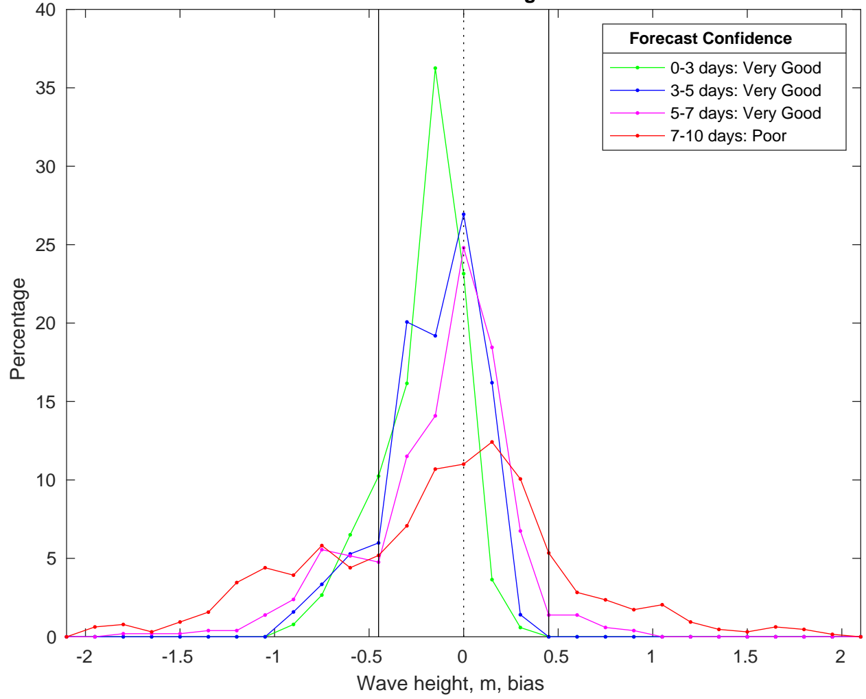
NDBC 42019 vs CMEMS Waves Bias Histogram: 16-Feb-2025
