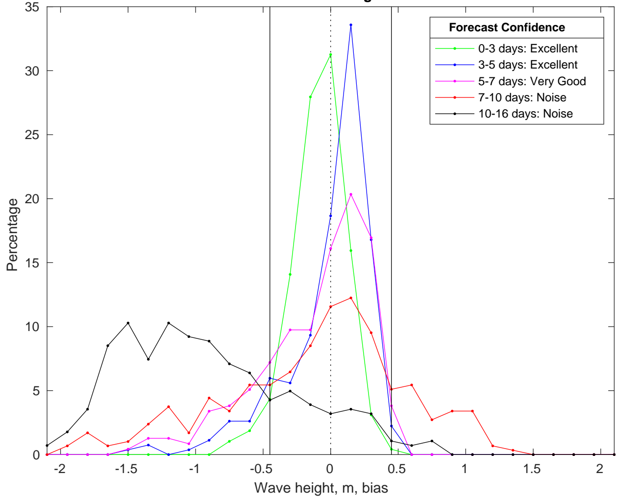
NDBC 42019 vs GFS Waves Bias Histogram: 16-Feb-2025
