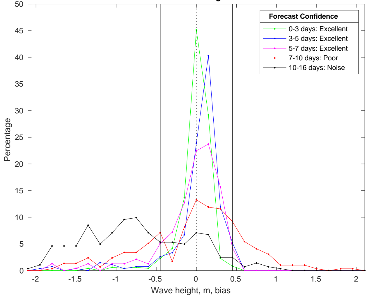
NDBC 42020 vs GFS Waves Bias Histogram: 16-Feb-2025
