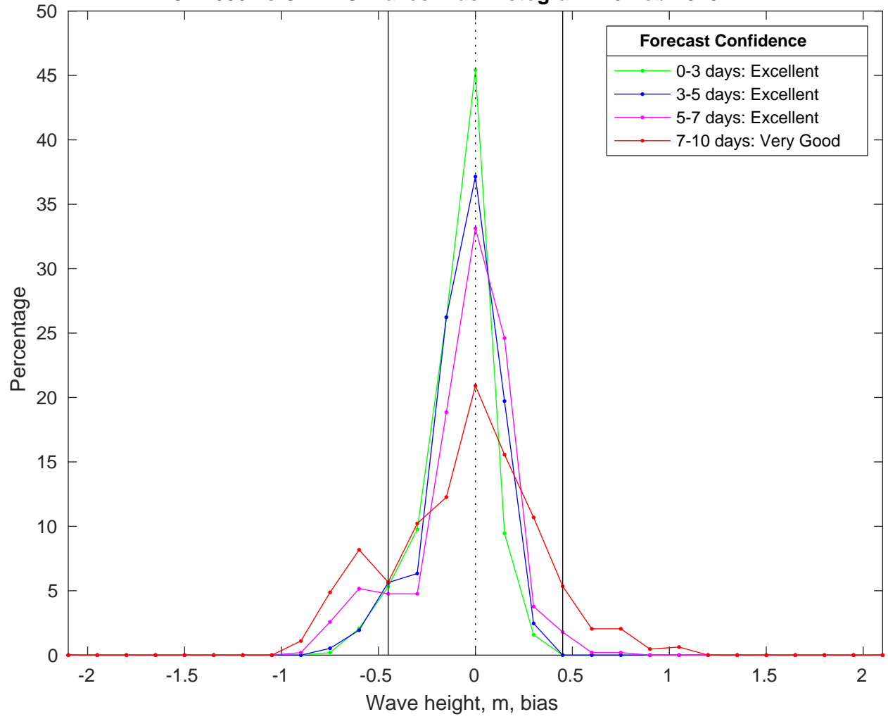
NDBC 42035 vs CMEMS Waves Bias Histogram: 16-Feb-2025
