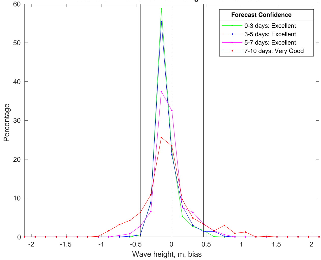
NDBC 42036 vs CMEMS Waves Bias Histogram: 16-Feb-2025
