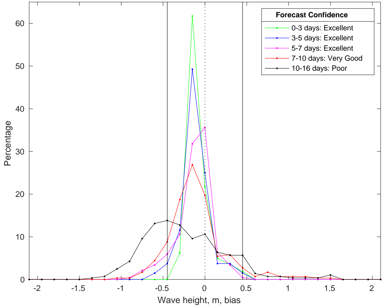
NDBC 42036 vs GFS Waves Bias Histogram: 16-Feb-2025
