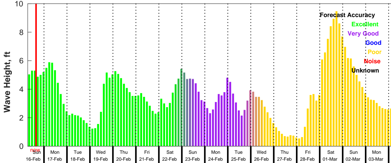
GFS Wave Forecast for NDBC 42036 from 16-Feb-2025 07:00:00 to 04-Mar-2025 07:00:00
