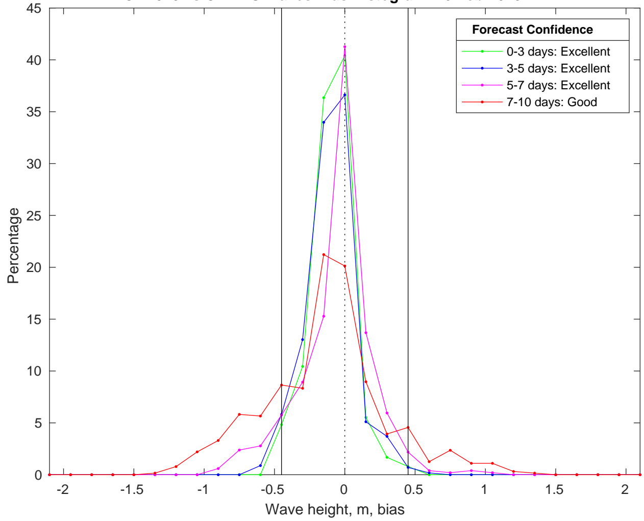
NDBC 42040 vs CMEMS Waves Bias Histogram: 16-Feb-2025
