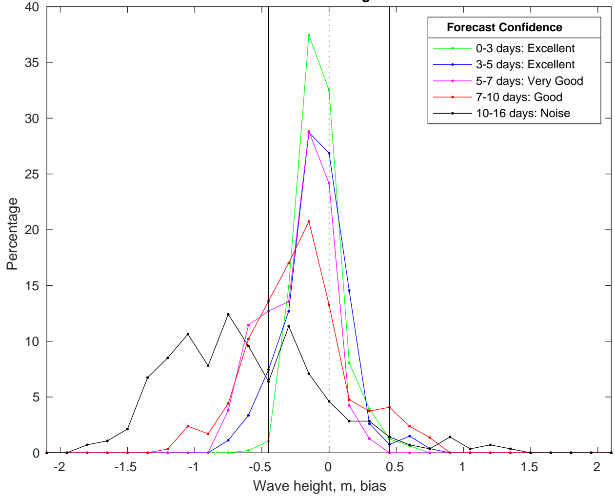
NDBC 42040 vs GFS Waves Bias Histogram: 16-Feb-2025
