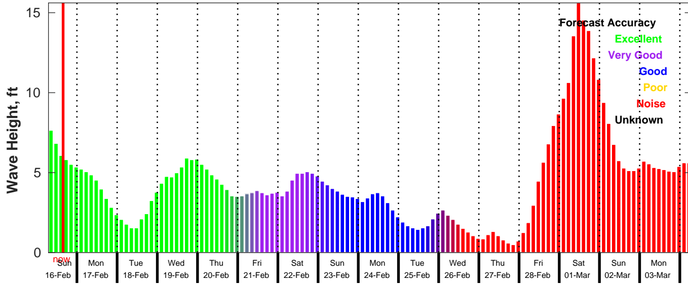
GFS Wave Forecast for NDBC 42040 from 16-Feb-2025 07:00:00 to 04-Mar-2025 07:00:00
