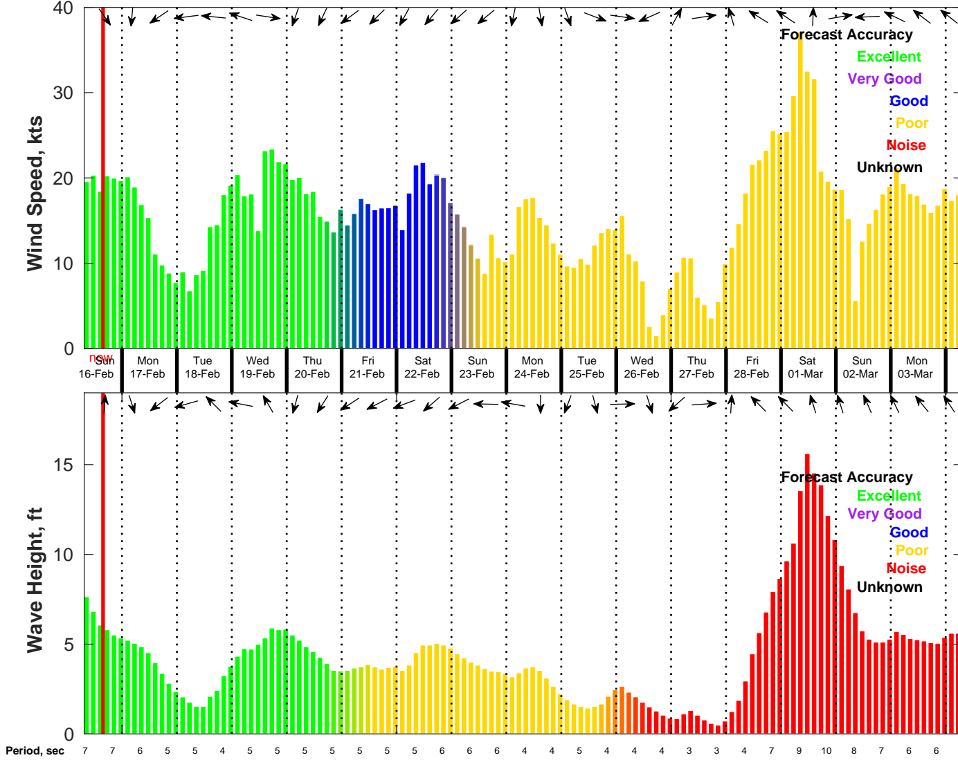
Wind & Wave Forecast for NDBC 42040 from 16-Feb-2025 07:00:00 to 04-Mar-2025 07:00:00
