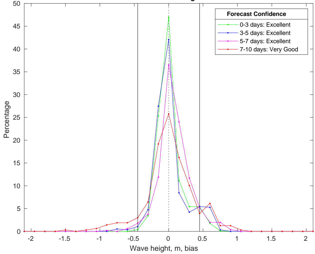
NDBC 42084 vs CMEMS Waves Bias Histogram: 16-Feb-2025
