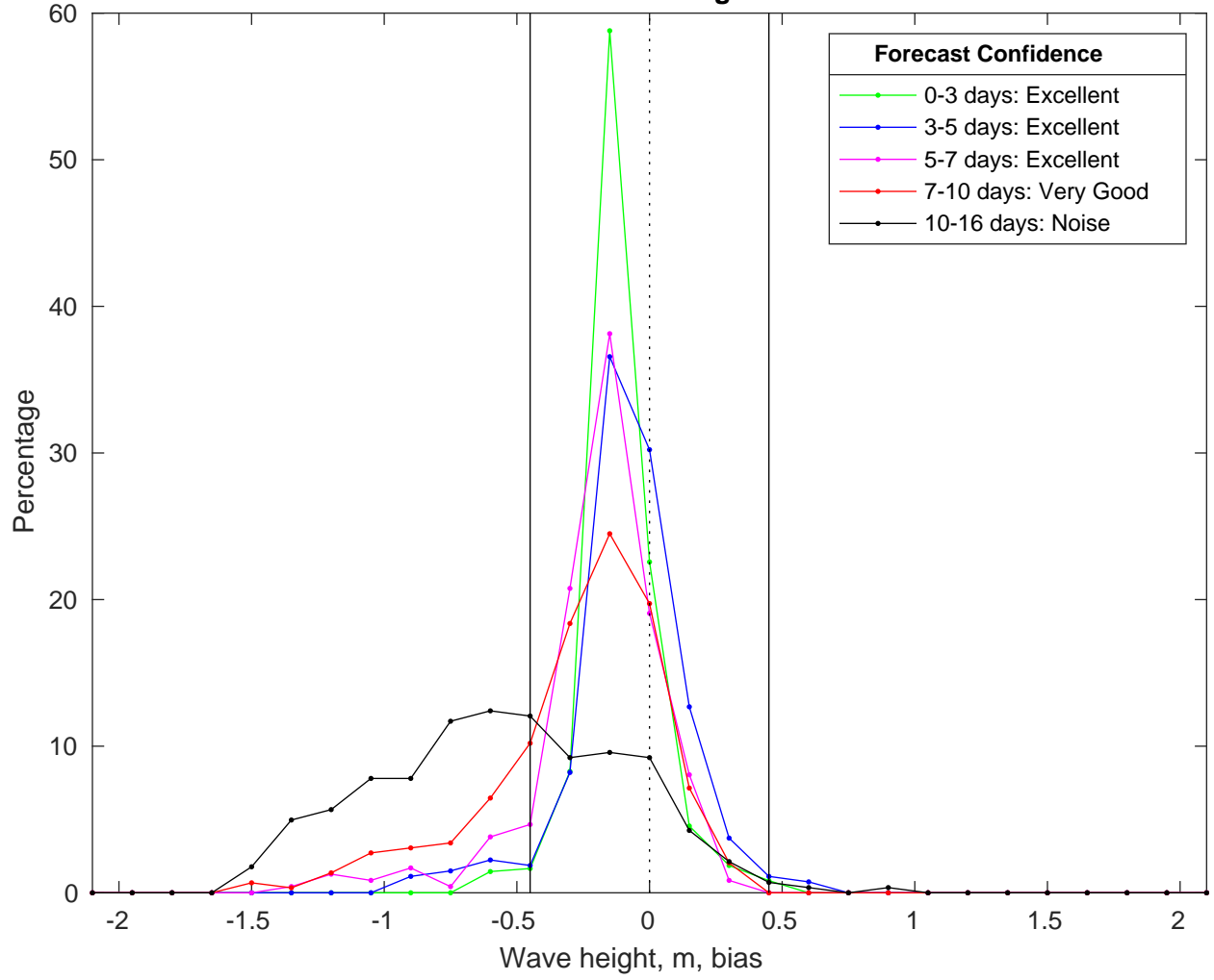
NDBC 42084 vs GFS Waves Bias Histogram: 16-Feb-2025
