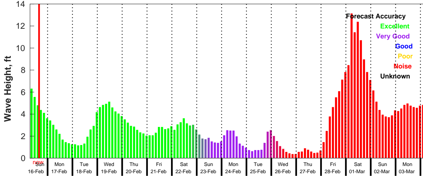
GFS Wave Forecast for NDBC 42084 from 16-Feb-2025 07:00:00 to 04-Mar-2025 07:00:00
