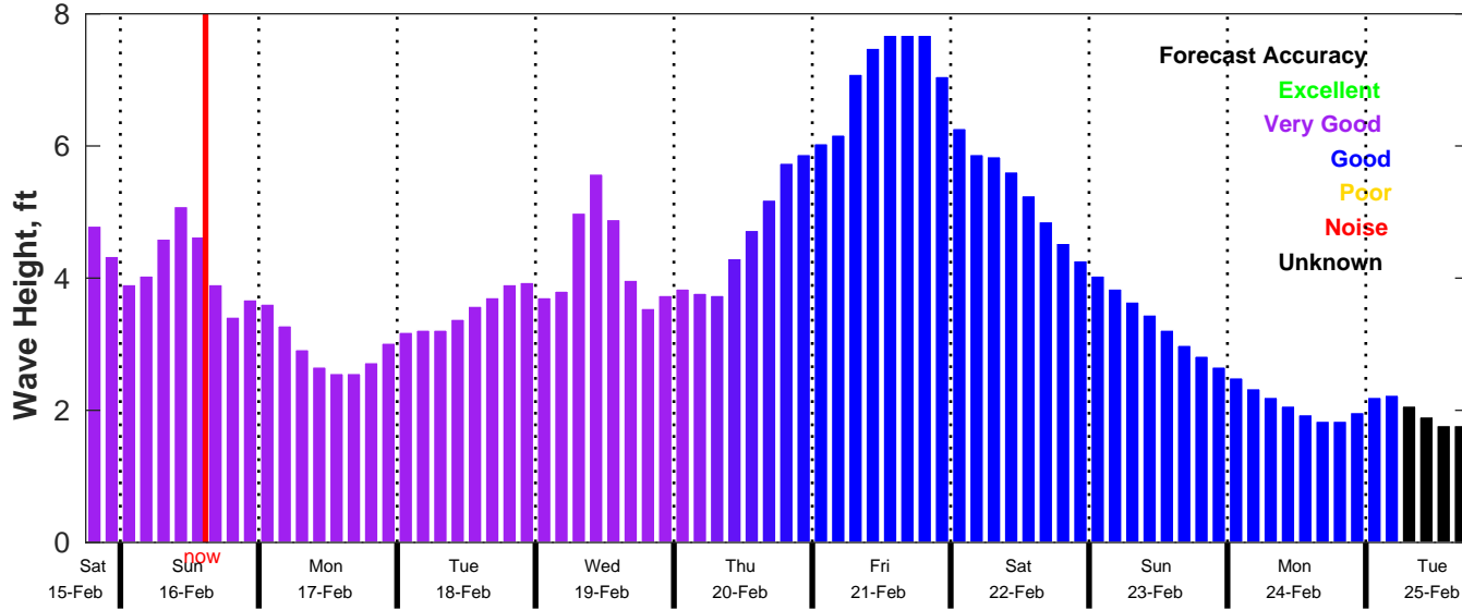
CMEMS Wave Forecast for NDBC 42092 from 15-Feb-2025 18:00:00 to 25-Feb-2025 18:00:00
