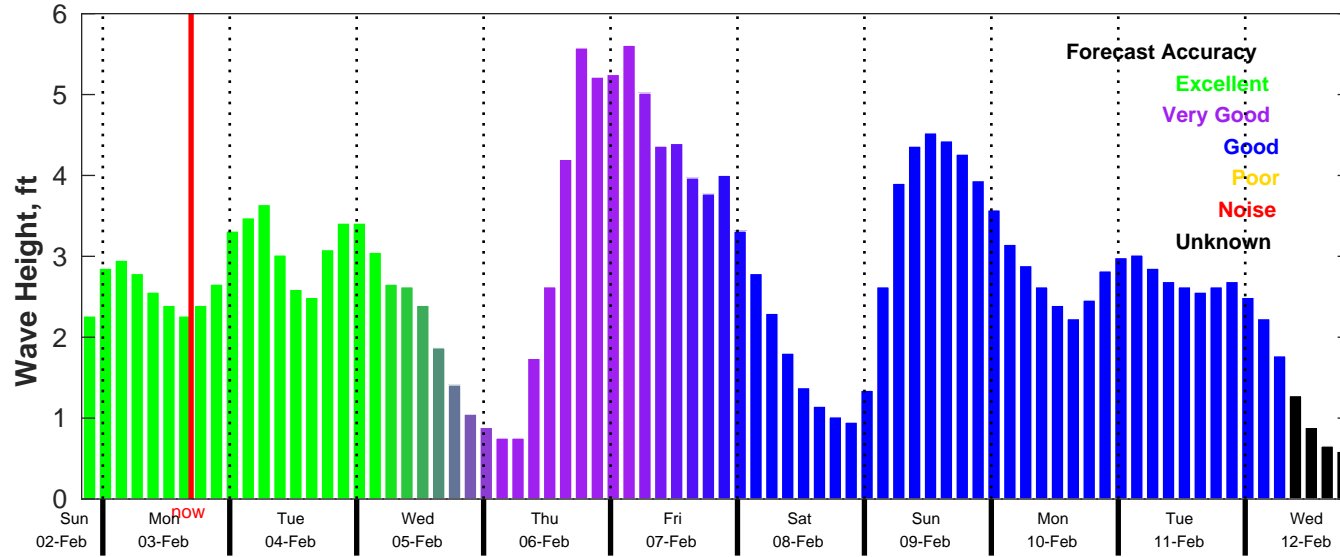
CMEMS Wave Forecast for NDBC 44020 from 02-Feb-2025 20:00:00 to 12-Feb-2025 20:00:00
