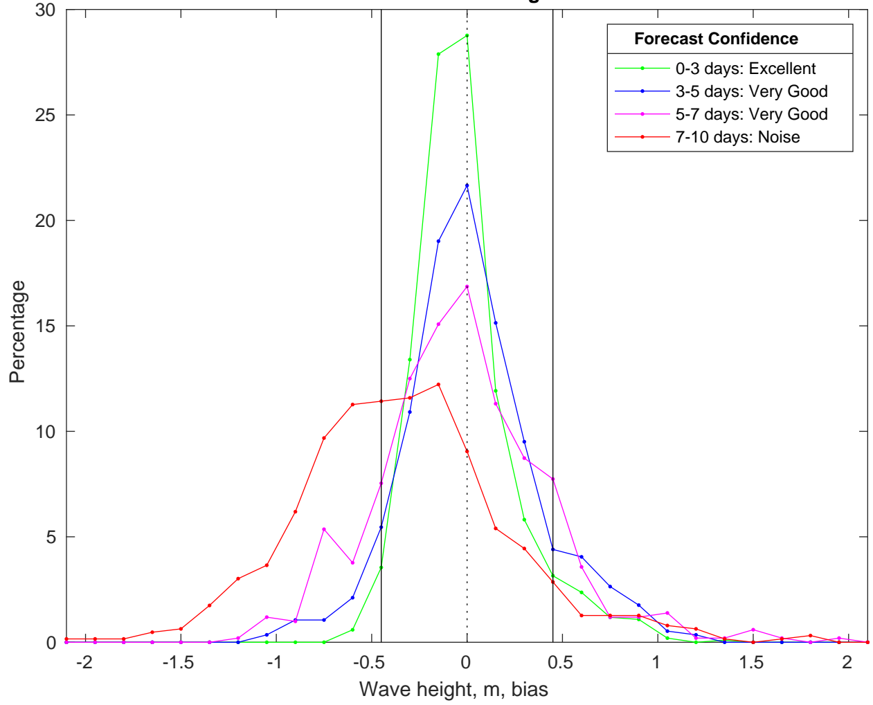
NDBC 46011 vs CMEMS Waves Bias Histogram: 16-Feb-2025
