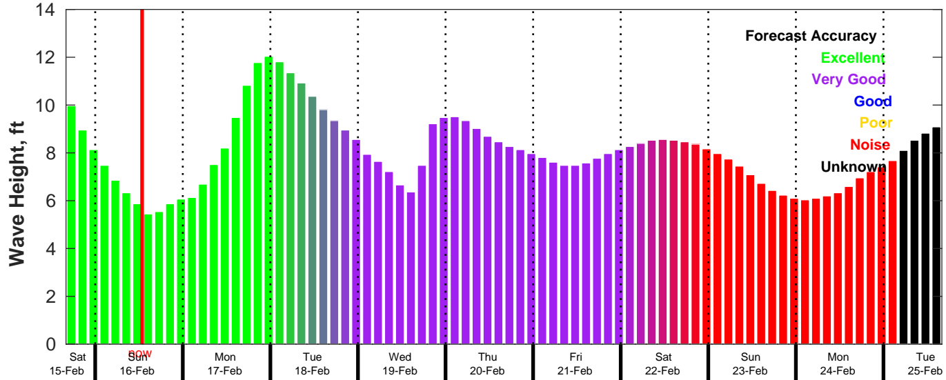
CMEMS Wave Forecast for NDBC 46011 from 15-Feb-2025 16:00:00 to 25-Feb-2025 16:00:00
