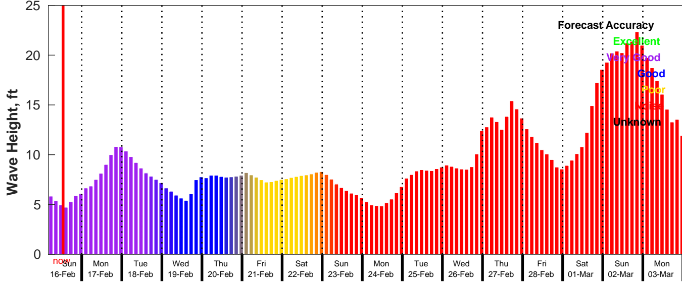
GFS Wave Forecast for NDBC 46011 from 16-Feb-2025 04:00:00 to 04-Mar-2025 04:00:00
