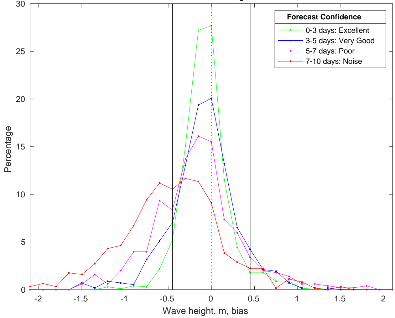
NDBC 46028 vs CMEMS Waves Bias Histogram: 16-Feb-2025
