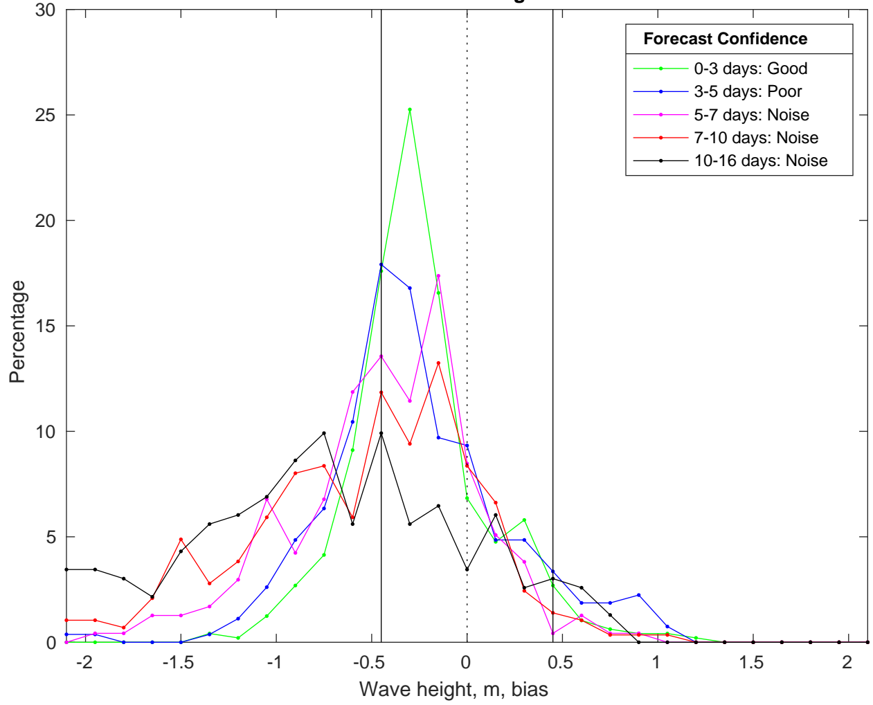
NDBC 46028 vs GFS Waves Bias Histogram: 16-Feb-2025
