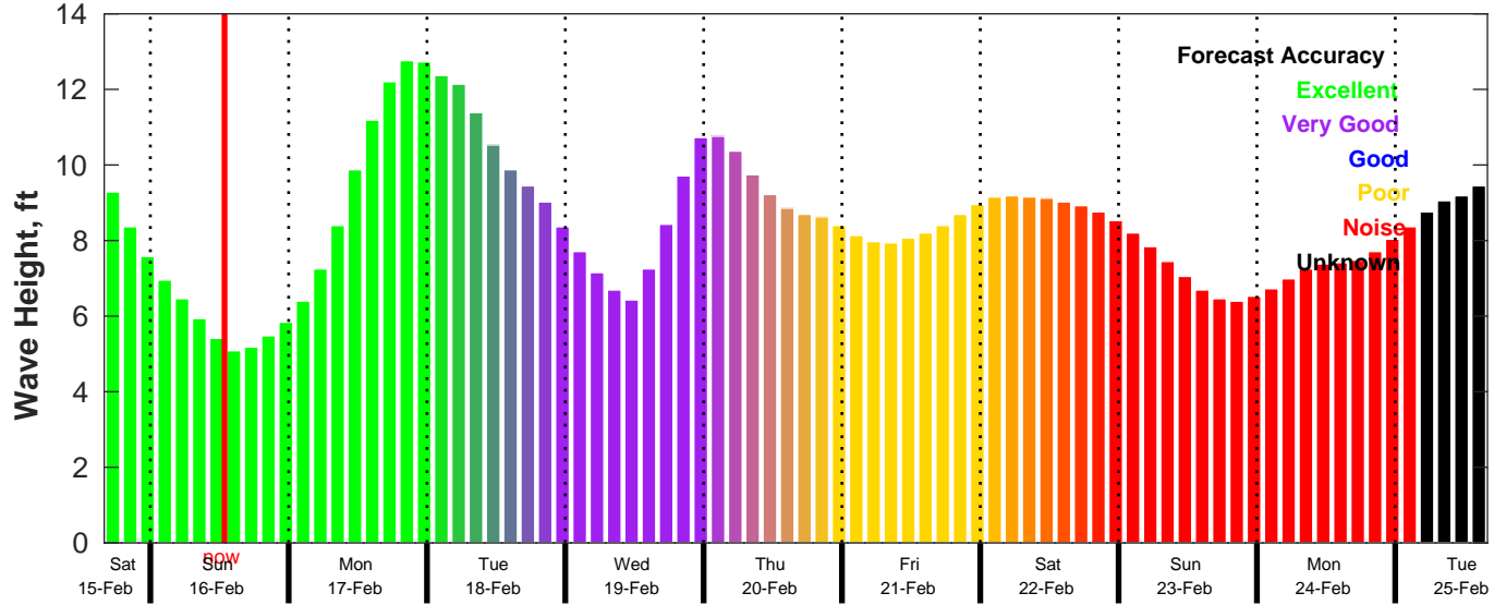
CMEMS Wave Forecast for NDBC 46028 from 15-Feb-2025 16:00:00 to 25-Feb-2025 16:00:00
