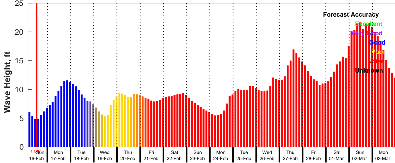
GFS Wave Forecast for NDBC 46028 from 16-Feb-2025 04:00:00 to 04-Mar-2025 04:00:00
