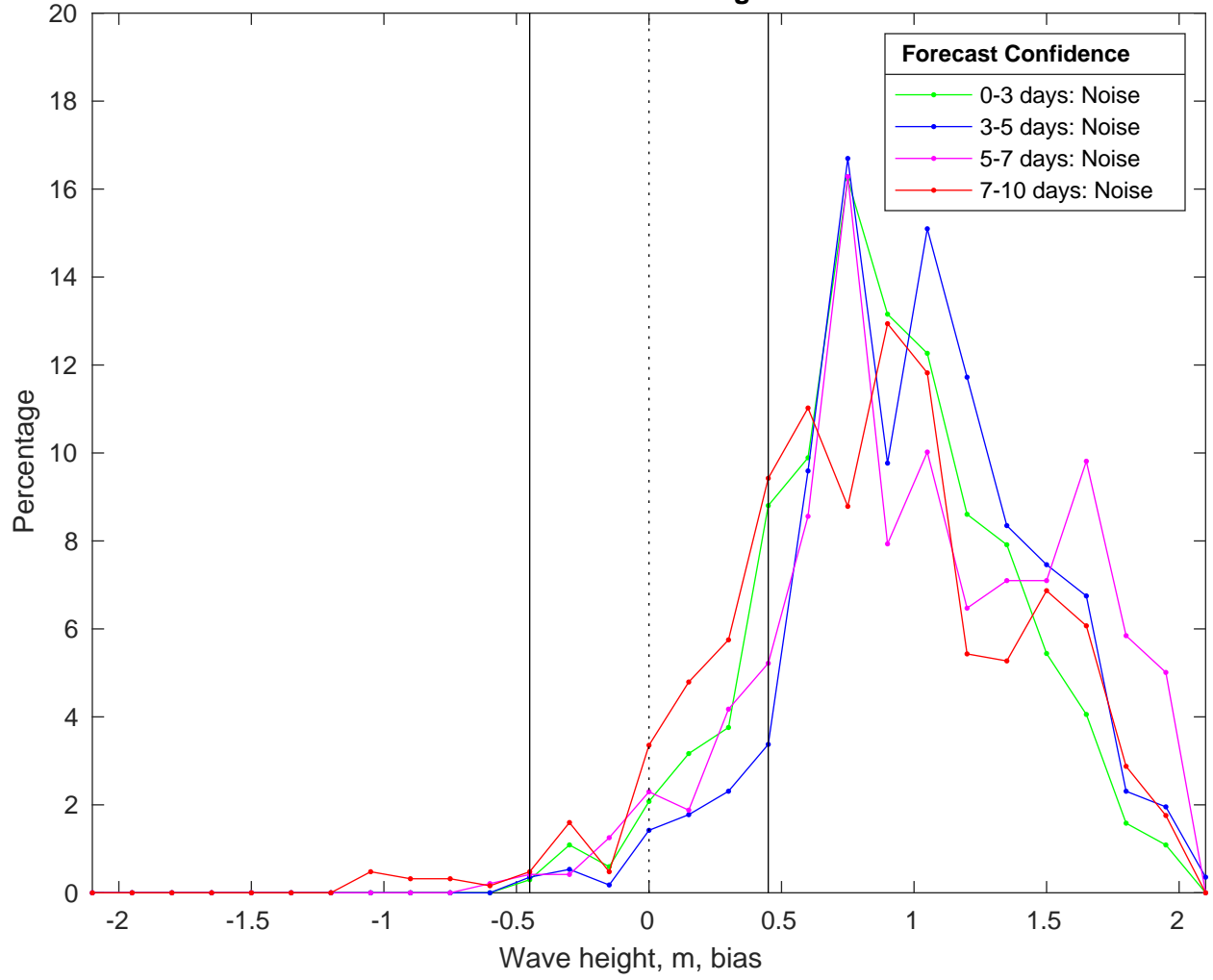
NDBC 46053 vs CMEMS Waves Bias Histogram: 16-Feb-2025
