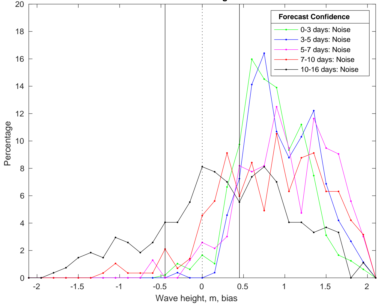
NDBC 46053 vs GFS Waves Bias Histogram: 16-Feb-2025
