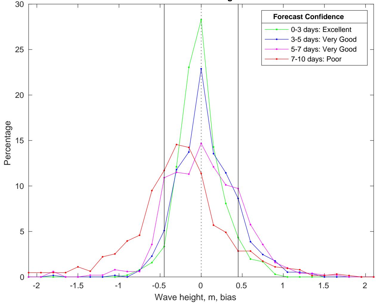
NDBC 46054 vs CMEMS Waves Bias Histogram: 16-Feb-2025
