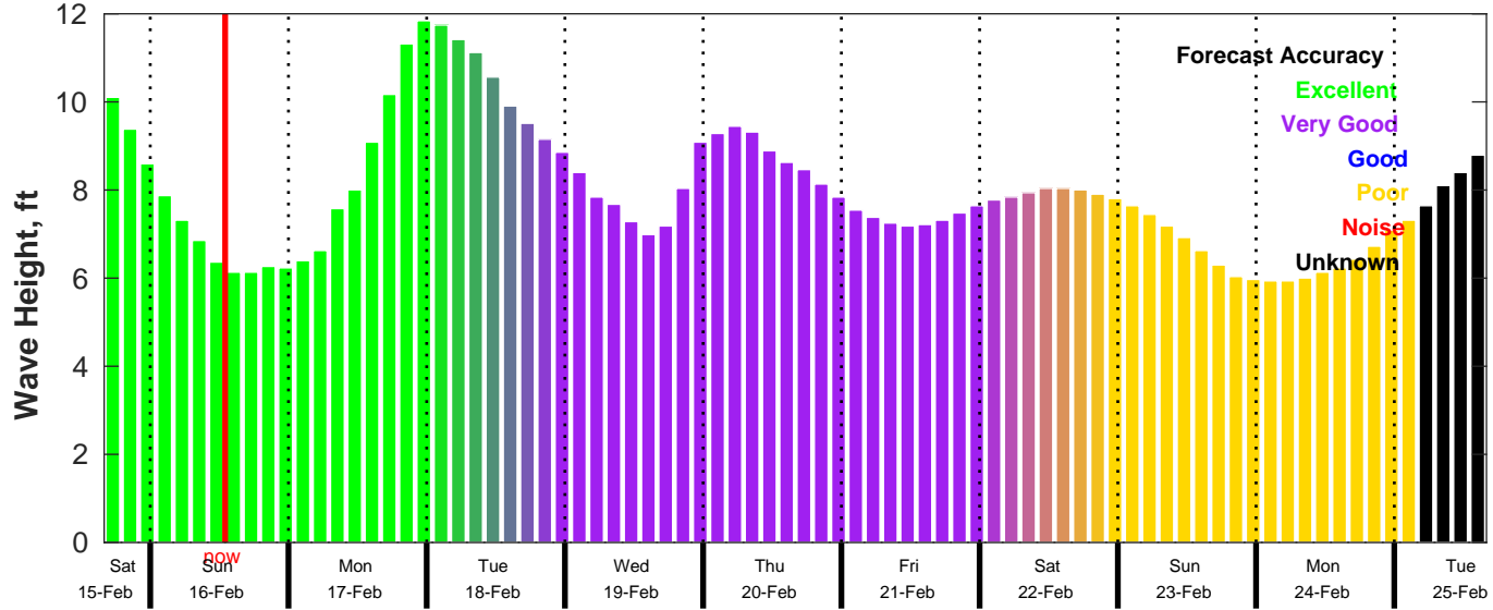
CMEMS Wave Forecast for NDBC 46054 from 15-Feb-2025 16:00:00 to 25-Feb-2025 16:00:00
