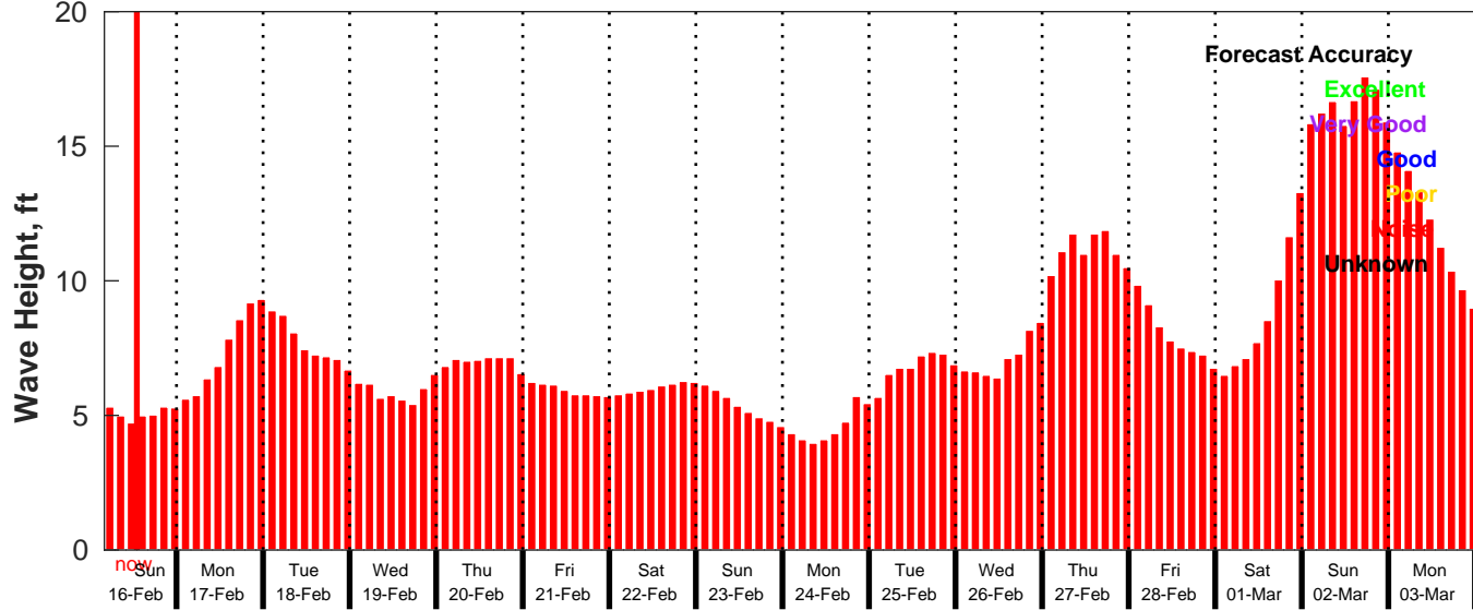
GFS Wave Forecast for NDBC 46054 from 16-Feb-2025 04:00:00 to 04-Mar-2025 04:00:00
